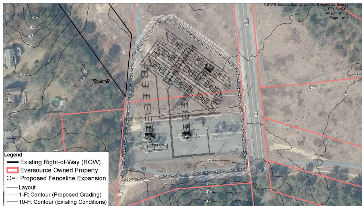
Figure 1. West Pond Substation Expansion Conceptual Layout
