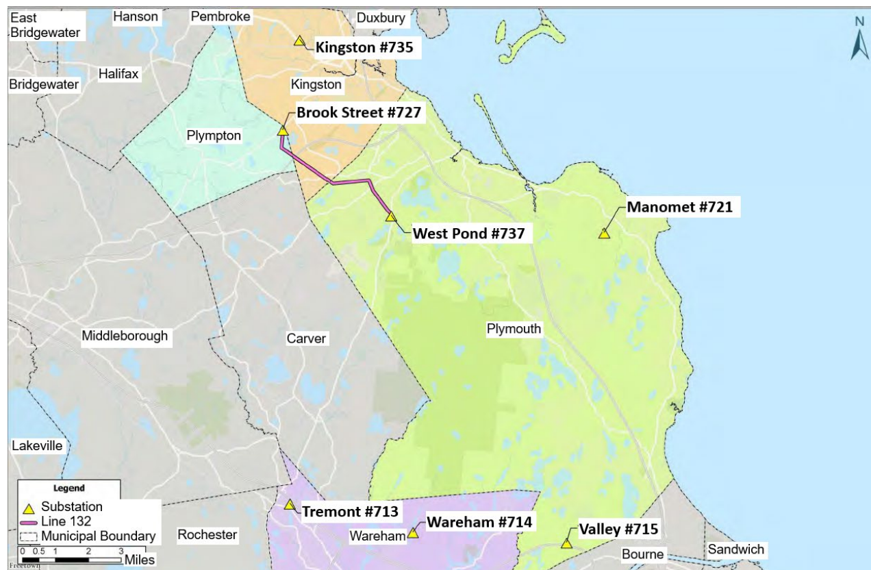
Figure 3. Plymouth Group Substations and Service Area
