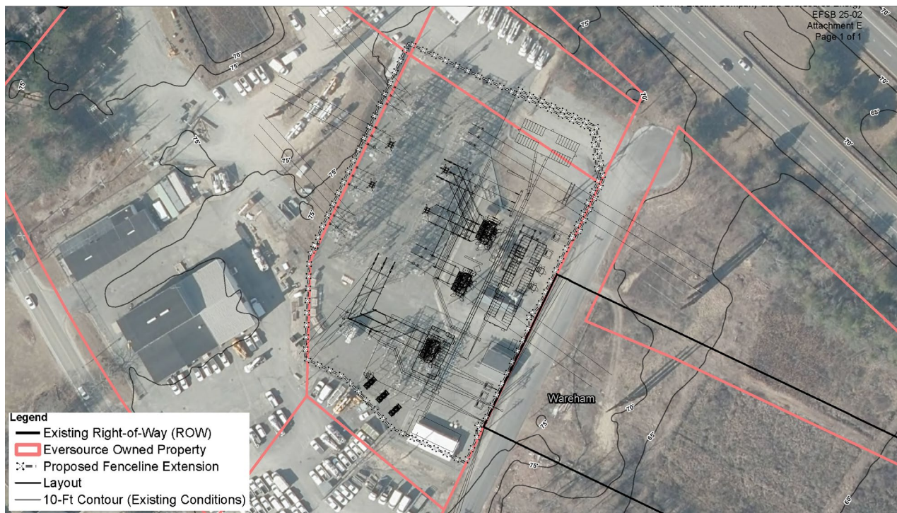
Figure 2. Tremont Substation Expansion Conceptual Layout
