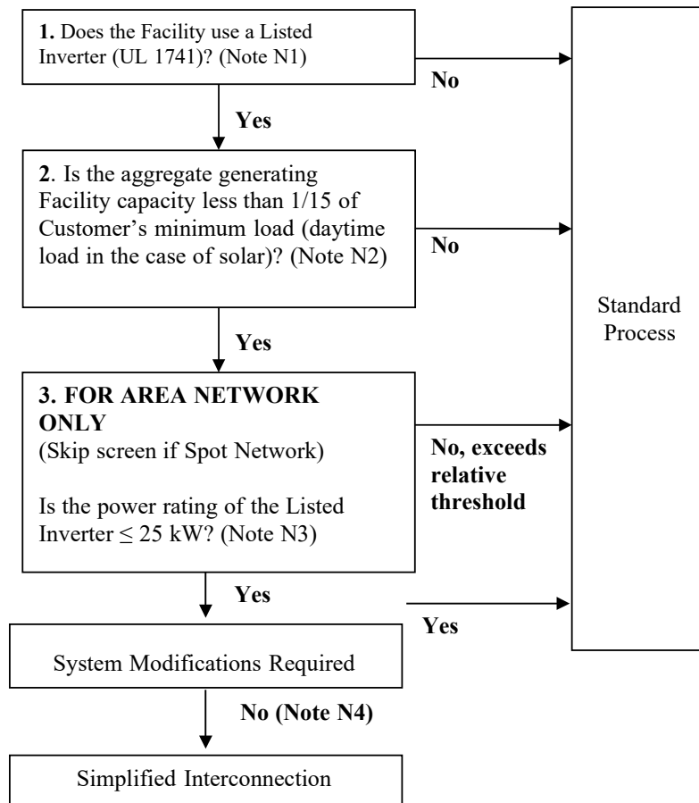
Figure 2 – Simplified Interconnection to Networks
